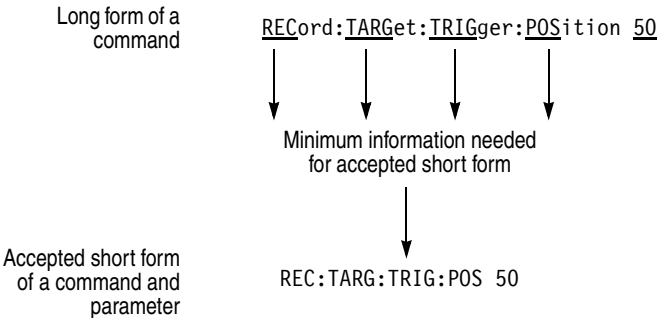
Figure 3-29: Example of abbreviating a command
