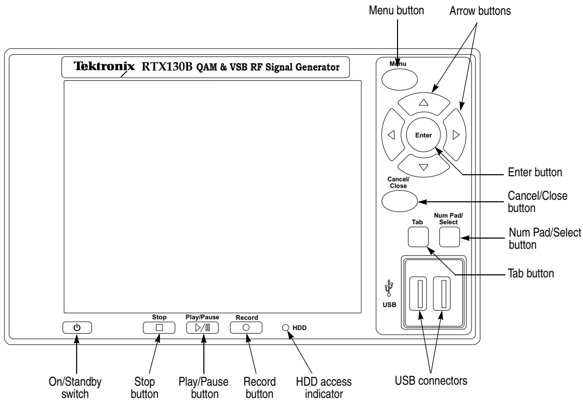
Figure 2-1: RTX130B front panel
