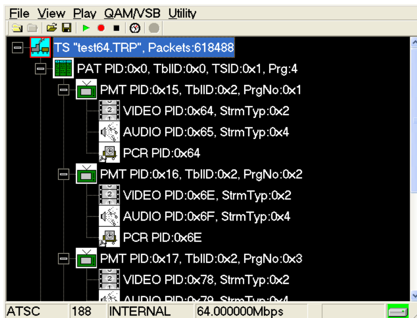
Figure 2-10: Hierarchy view of the transport stream file
