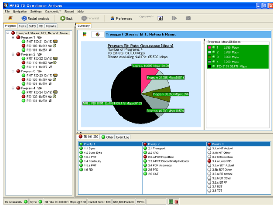
Figure 2-12: Transport stream display from an MPEG test system
